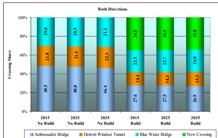
Figure 6-6. Total Crossing Share with Multinomial Logit Model
