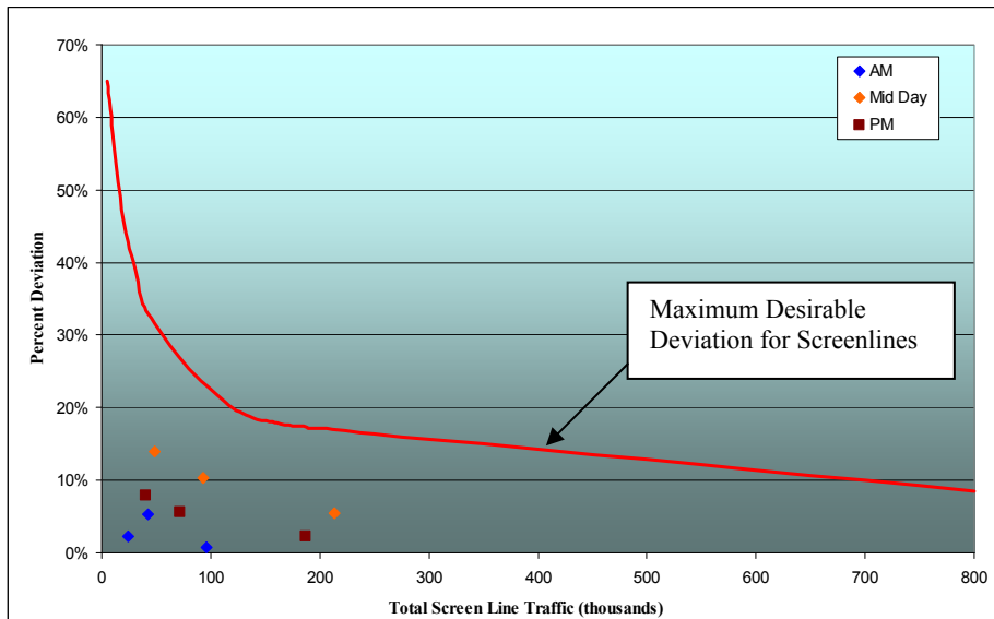
Figure 5-10. Travel Demand Model Validation Results
