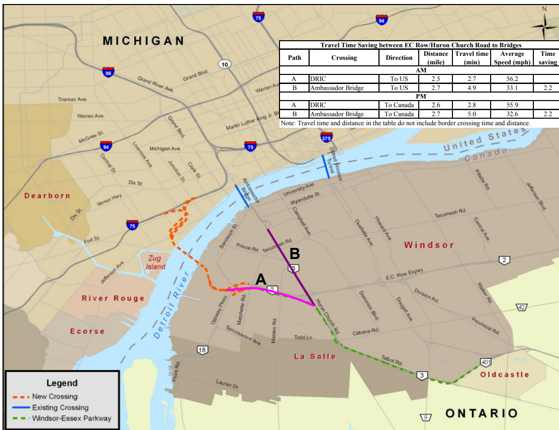
Figure 6-9. 2025 Travel Time Comparison between Huron Church Road/E.C. Row Expressway and Bridges
