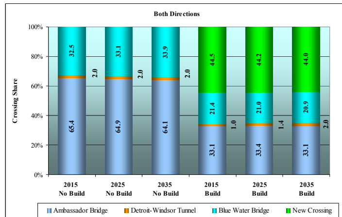
Figure 6-5. Commercial Vehicle Crossing Share with Multinomial Logit Model
