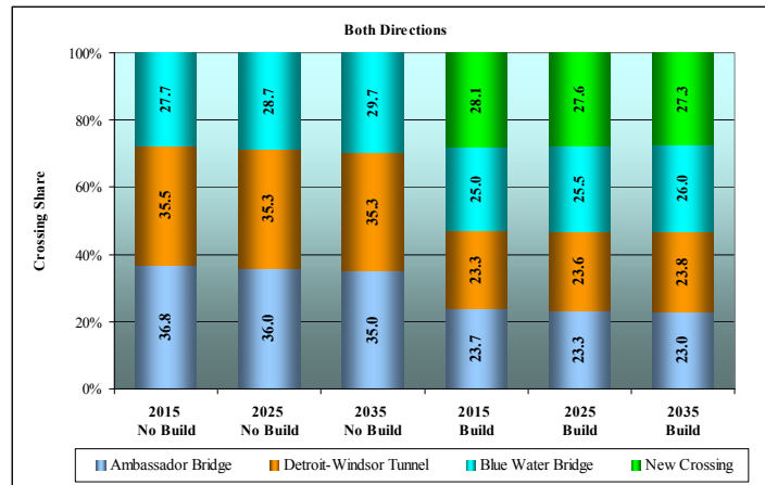
Figure 6-4. Passenger Car Crossing Share with Multinomial Logit Model
